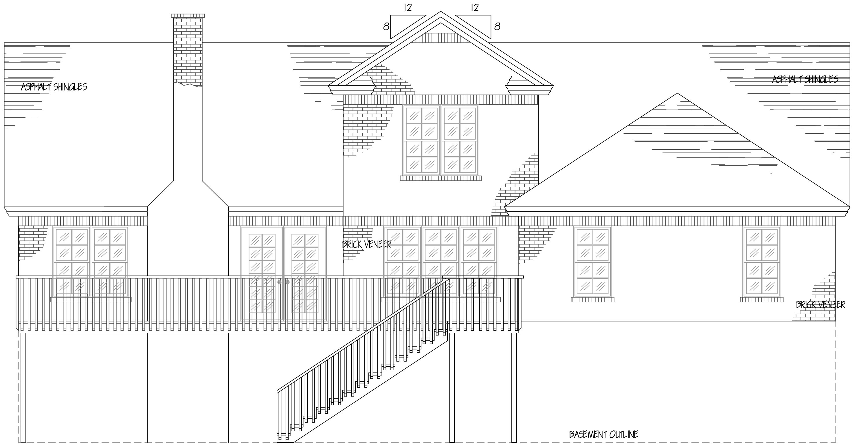
REAR ELEVATION
