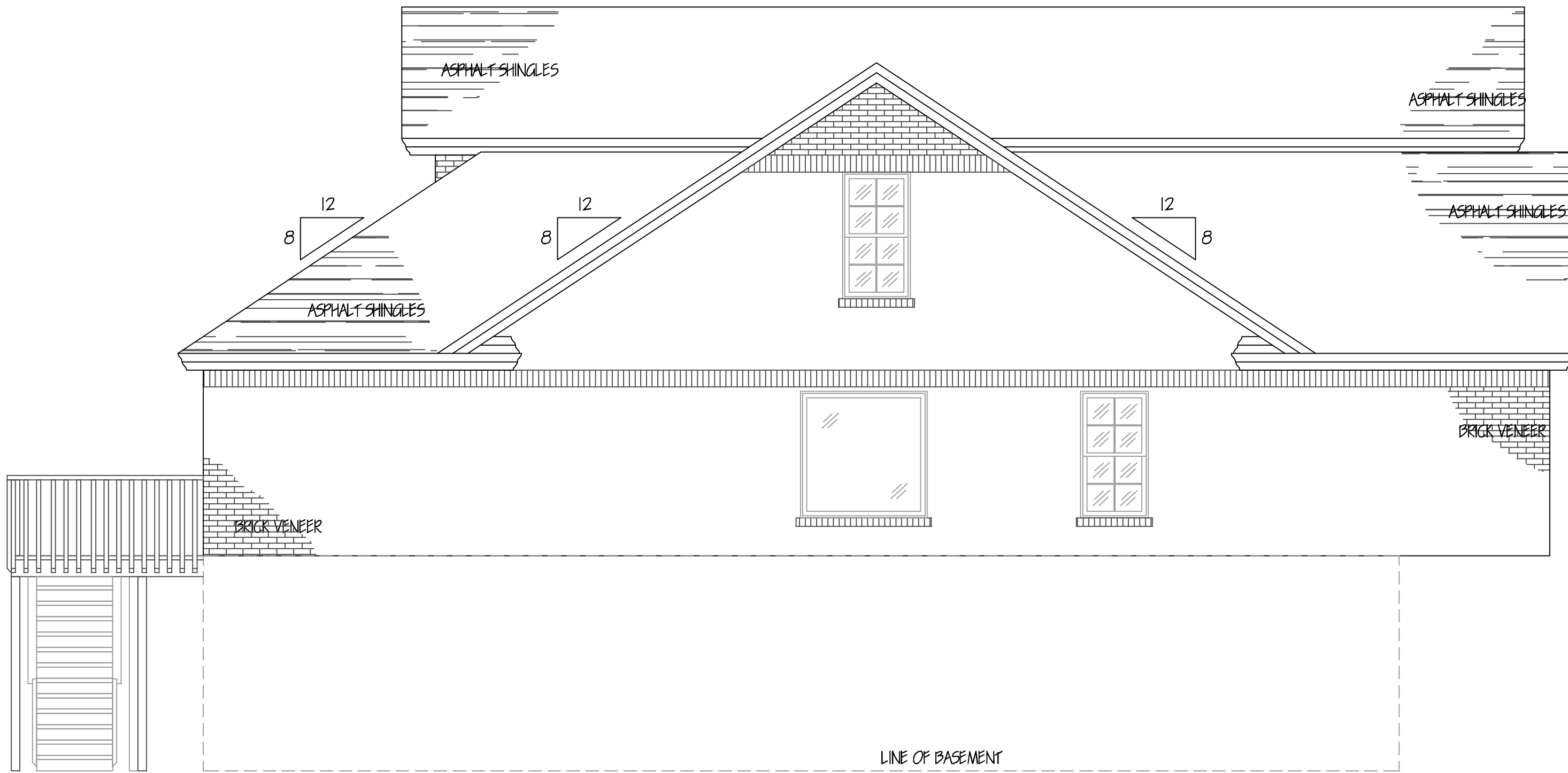
LEFT ELEVATION
