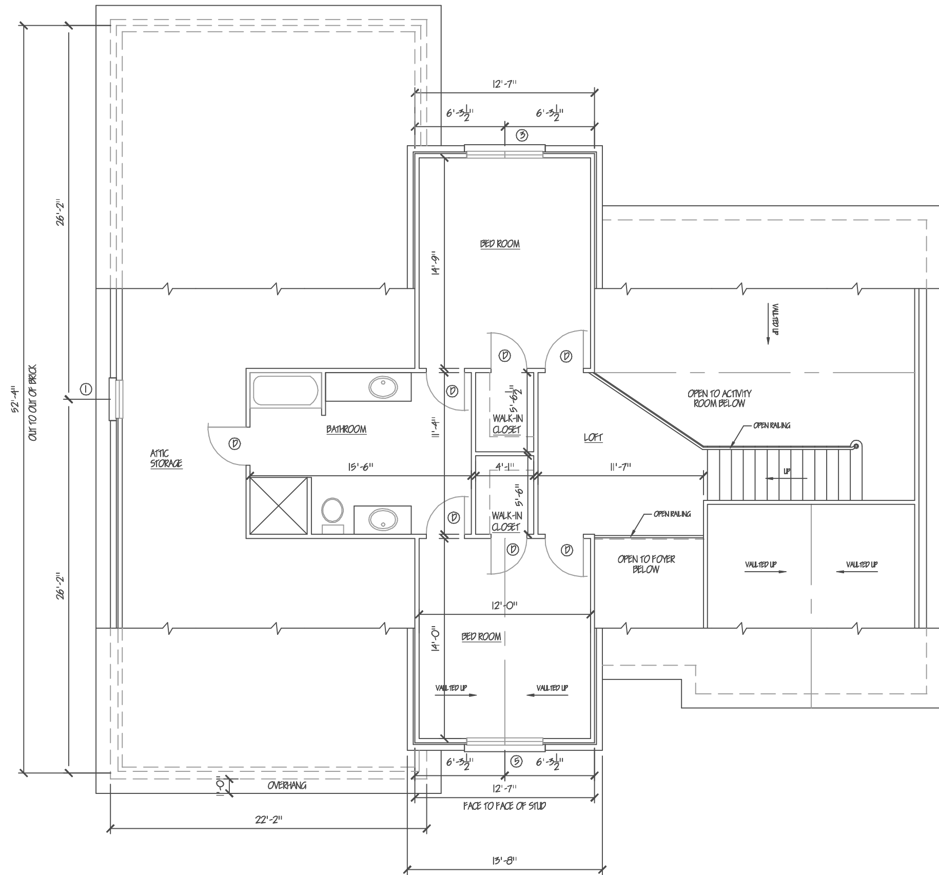
SECOND FLOOR SCALE: 1/4" = 1'-0"
